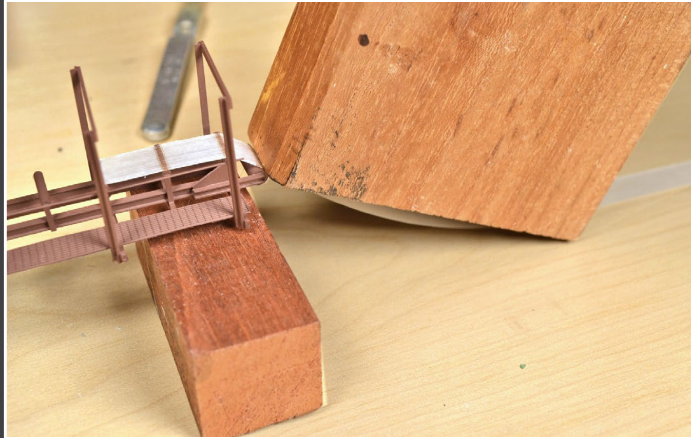
19: Adding the conveyor belt to the three top rollers.
