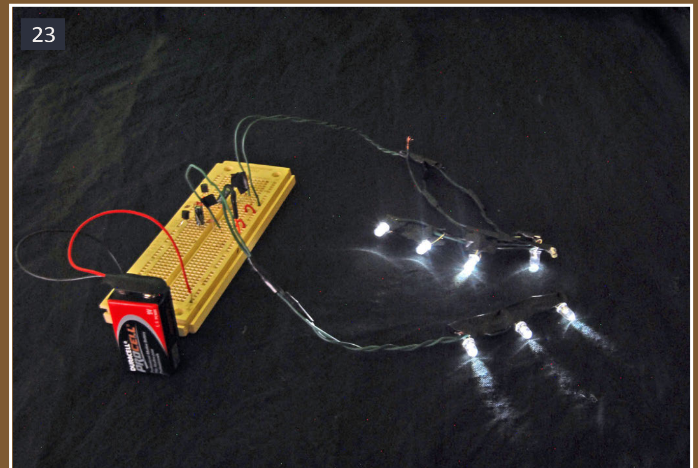
23: Testing the circuit.
