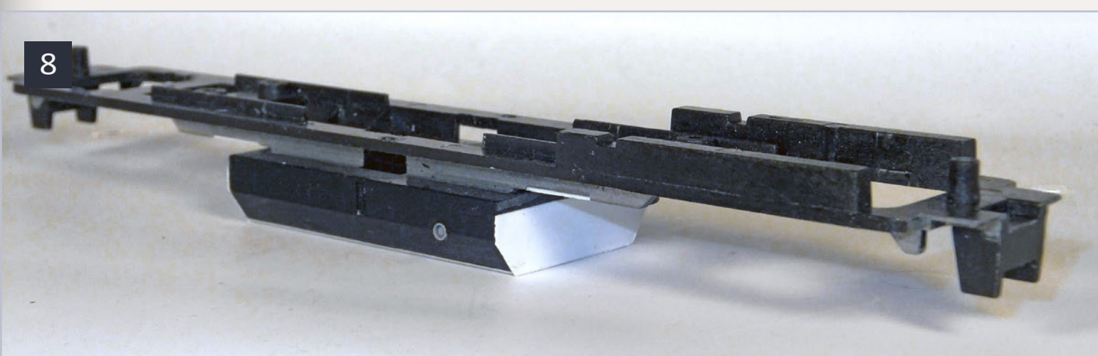
8: Brian Banna's chassis modifications include permanently mounting the fuel tank to the chassis after removing the cast-on air tanks, and drilling holes in the bottom to permit access to the motor mounting screws. He applied new ends and fuel gauges to the tank, and milled the frame rails. Most of this is similar to changes I made on my U18B that was featured in Model Railroad Hobbyist in July 2010.
