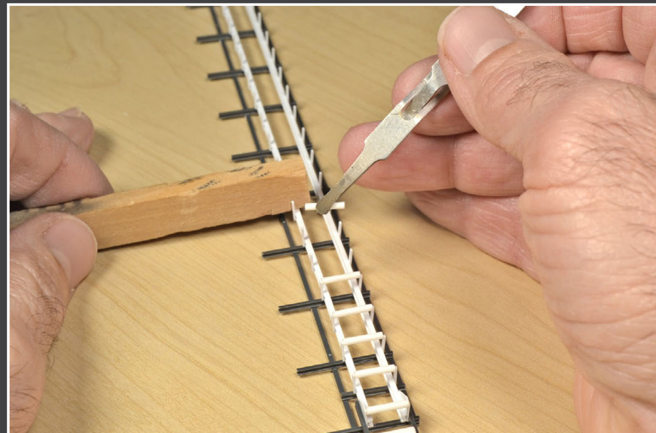
14: Adding the rollers.
