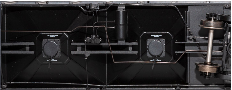
35. CABX 580772, closeup of brake and underframe details.
