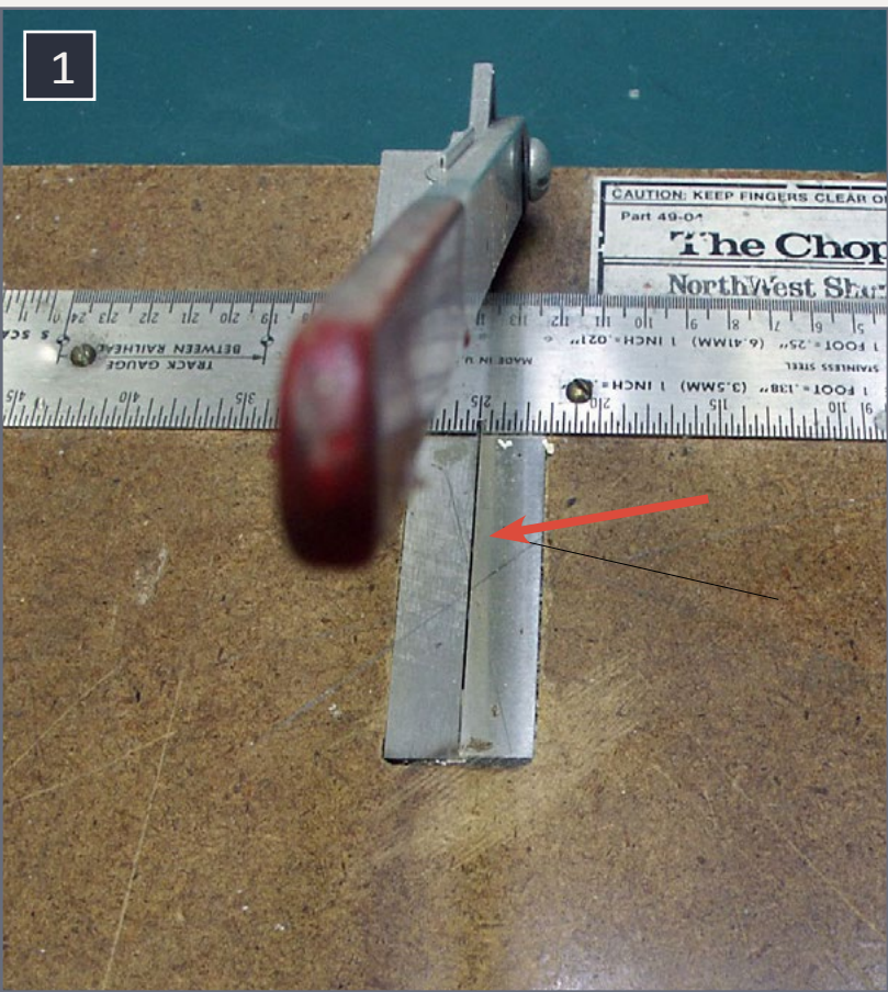
1. This is my Chopper that I modified. Two pieces of tool steel were placed on either side of the blade, creating a slot for the blade to rest in.
