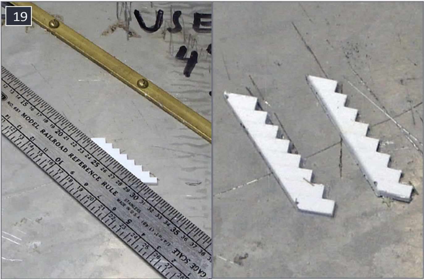
19. The 4 x 8's are cut down the center creating the two stringers required for a set of stairs.
