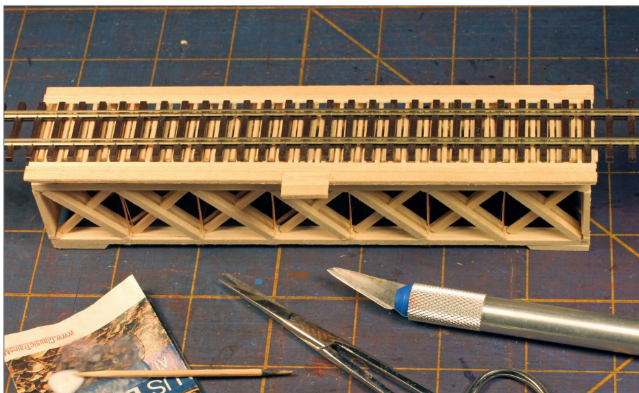
18. Test-fitting HOn3 flex track on the deck.
