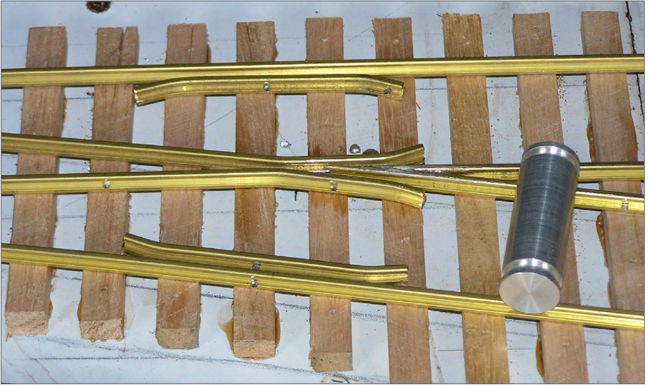
18. The gauge is checked on the diverging route.
