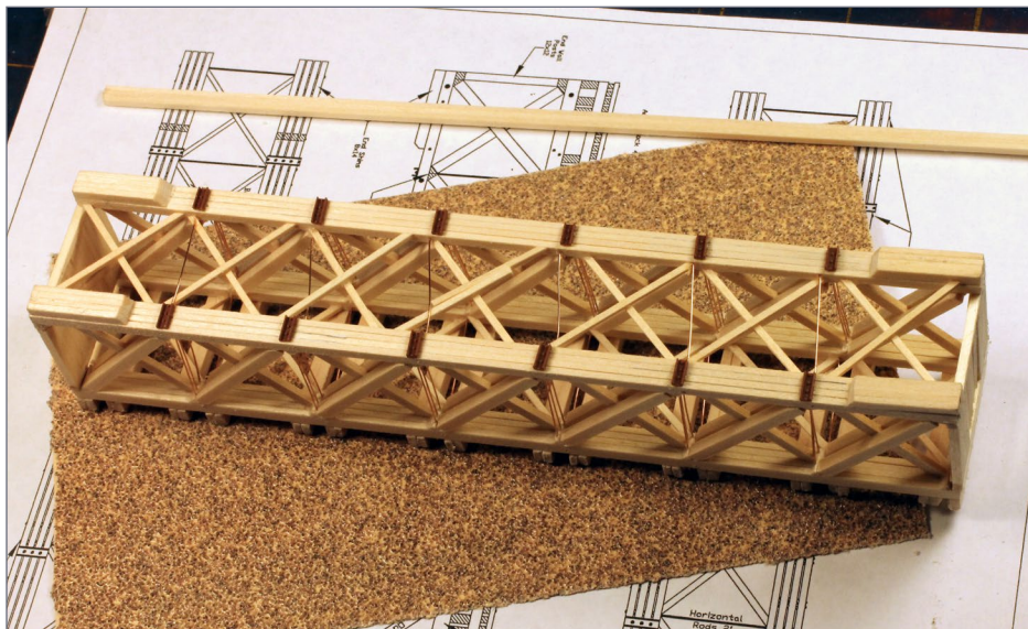
16. Make sure the deck supports are absolutely flat before gluing on the decking.
