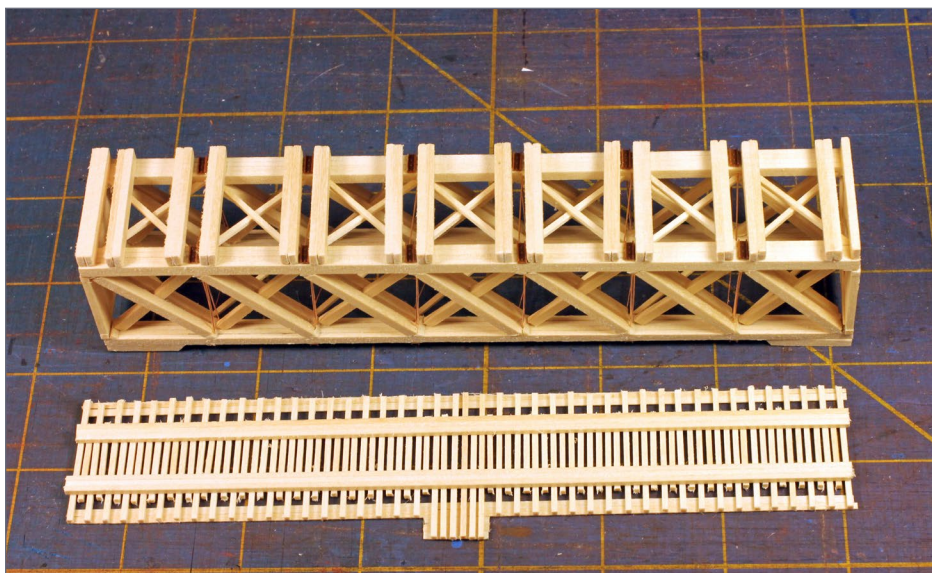
15. The decking and box structure completed.
