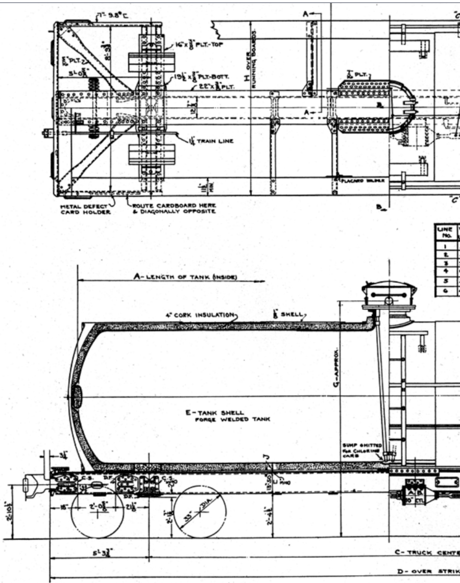
17. Drawing of an ICC 105A tank car, showing insulation thickness and valve bonnet, together with the education pipe by which cargo can be pumped out of the car, and the small sump located below that pipe to permit effective emptying of the car.
