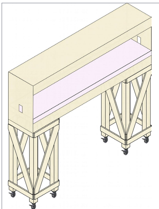
7. Complete shadowbox module section, mounted on movable supports.
